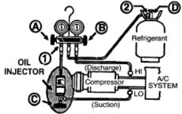
ADDING OIL OR CONDITIONER TO OPERATING (CHARGED) SYSTEM
