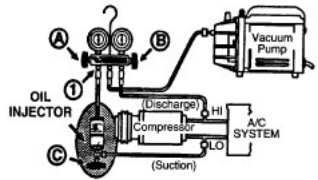
ADDING OIL OR CONDITIONER TO DISCHARGED SYSTEM
